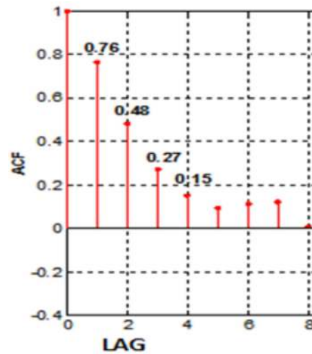
Fig 5(b) Autocorrelation
