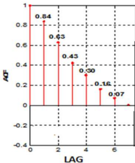
Fig. 4 (b) Autocorrelation
